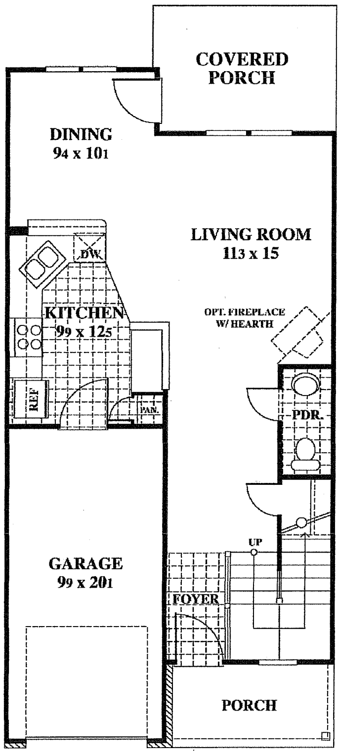
UNIT - D FIRST FLOOR PLAN
