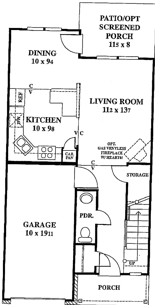
FIRST FLOOR - UNIT BII
